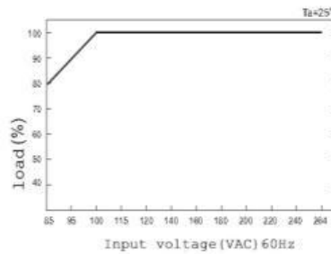
Static Characteristics(12V)
