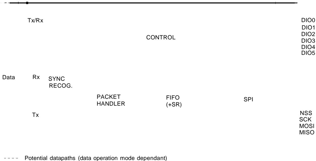
Figure 25. RFM95/96/98(W) Data Processing Conceptual View
