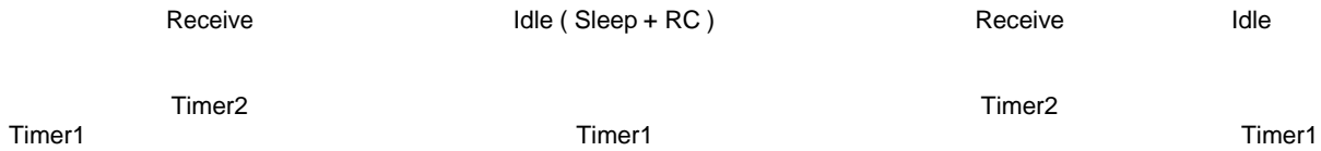
Figure 45. Listen Mode with No Preamble Received
