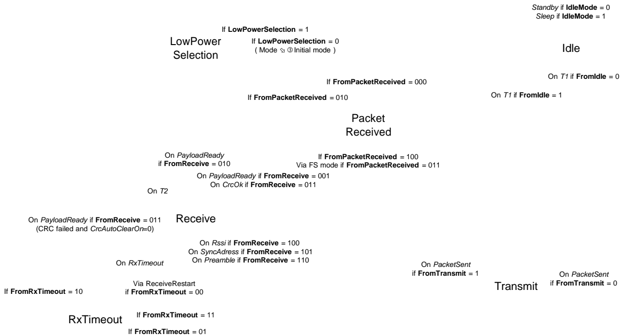
Figure 24. Sequencer State Machine
