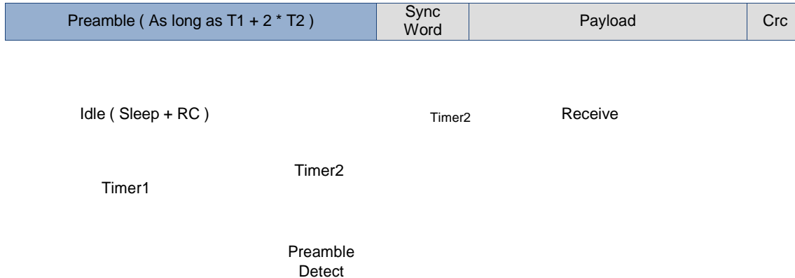
Figure 46. Listen Mode with Preamble Received
