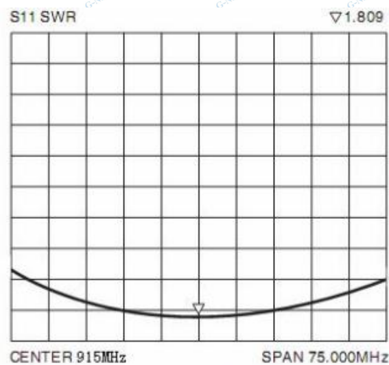
Typical VSWR
